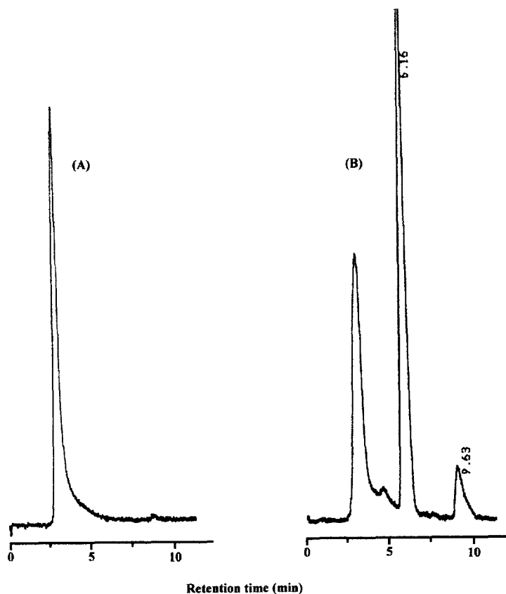
Fig. 2. Chromatograms of plasma extracts. (A) Blank human plasma, (B) human plasma spiked with 10 ng/ml of megazol and 500 ng of tinidazol.
